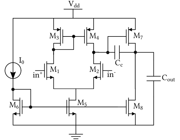
Fig. 11. Circuit schematic of a two-stage op-amp.
