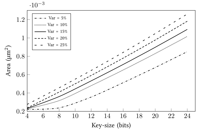
Fig. 17. Relation between the key size and the area of an op-amp obfuscated using the vector-based obfuscation technique for different percentage variation of both the target transistor size and the obfuscation transistor size.
