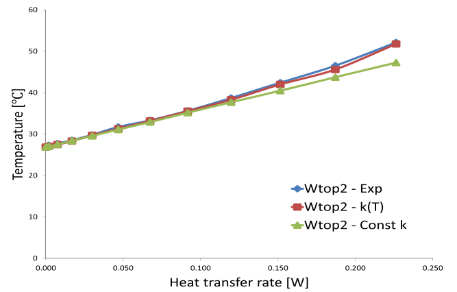
Fig. 11. Comparison of temperatures for a diagonal path (length = 1300 μm).
