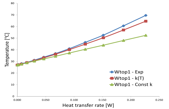
Fig. 10. Comparison of temperatures for a vertical path (length = 10 μm).
