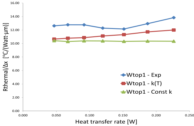
Fig. 13. Comparison of thermal resistance per unit length for a vertical path (length = 10 \mu\text{m} ).
