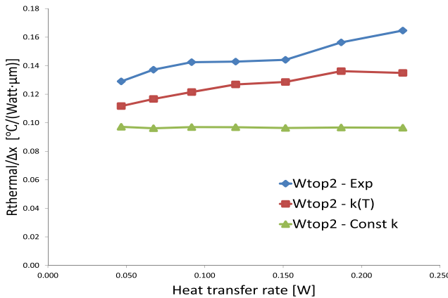
Fig. 14. Comparison of thermal resistance per unit length for a diagonal path (length = 1300 \mu\text{m} ).
