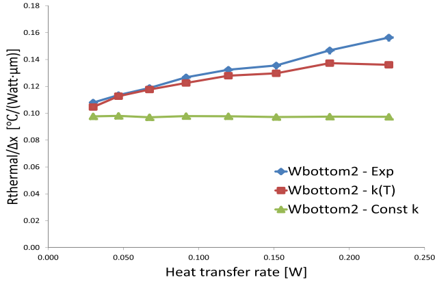
Fig. 12. Comparison of thermal resistance per unit length for a horizontal path (length = 1300 \mu\text{m} ).
