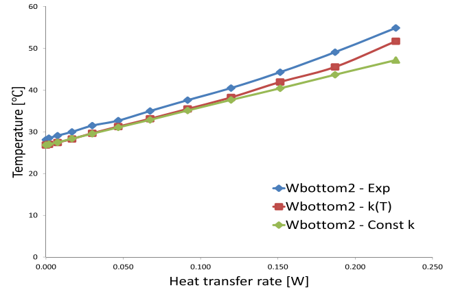
Fig. 9. Comparison of temperatures for a horizontal path (length = 1300 μm).
