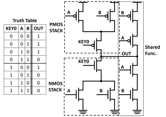
Fig. 3: Stack-based topology implementing a NAND or NOR gate depending on the value of KEY0.
