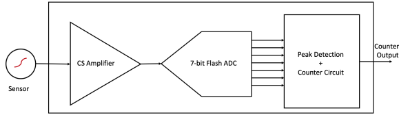
Figure 1: AMS circuit obfuscated with the proposed technique.
